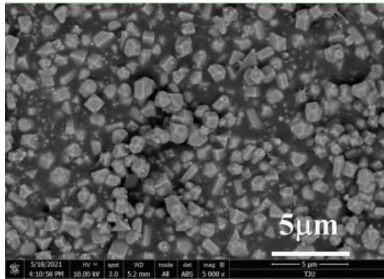
Figure S1. SEM image of the Cu powder.
