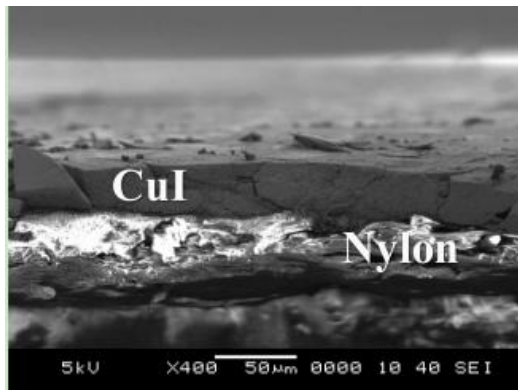
Figure S2. SEM image of the cross section of the HP-film.
