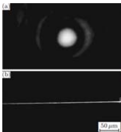
Fig. 2. Waveguide formed in the fused silica glass using 800 nm, 120 fs and 1 kHz mode-locked pulses with an average power of 6 mW through a microscope objective ( \text{NA} = 0.3 , 10\times ) by moving the sample at 30 \mu\text{m/s} . For this case, \Delta n has the maximum of 0.008. (a) Far-field mode pattern at 632.8 nm output of induced waveguide in fused silica glass. (b) Image of a waveguide line guiding 632.8 nm light in fused silica glass.
