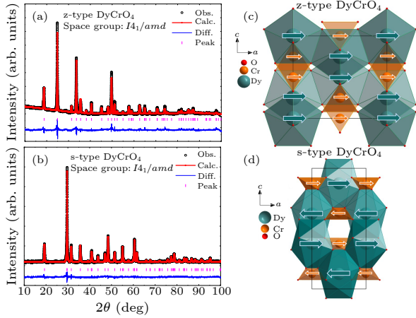
Fig. 1. Rietveld refinement of x-ray powder diffraction patterns of (a) z-type DyCrO 4 (Cu K\alpha ) and (b) s-type DyCrO 4 at room temperature. (c) The zircon-type and (d) scheelite-type crystal structures of DyCrO 4 . Directions of spin moments are indicated by arrows.
