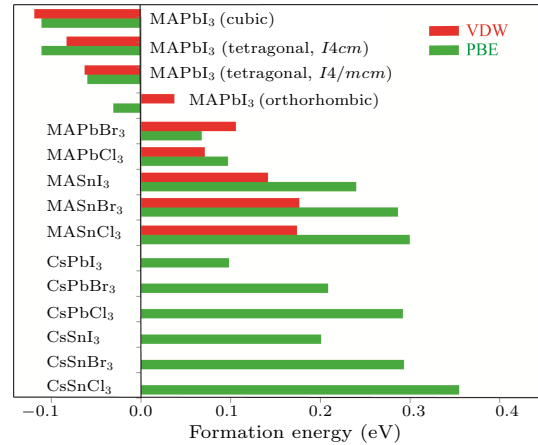
Fig. 2. The calculated energy cost of the phase separation of \text{ABX}_3 ( A = \text{CH}_3\text{NH}_3 , \text{Cs} , B = \text{Pb} , \text{Sn} , X = \text{I} , \text{Br} , \text{Cl} ) in their orthorhombic structure. For \text{CH}_3\text{NH}_3\text{PbI}_3 , the results of all the three structures are plotted. For the organic-inorganic hybrid perovskites, the results from both the vdW-TS and PBE functionals are plotted. Positive number indicates that the compound is stable at T = 0\text{K} .
