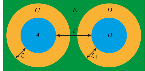
Fig. 2. A two-dimensional illustration of short-range entanglement of an eigenstate of an MBL system. If the separation distance l between regions A and B is much larger than twice the characteristic length \xi_+ of the raising/lowering operators, there will be no entanglement or correlation between regions A and B because region E can be unitarily transformed into vacuum without affecting regions A and B .
