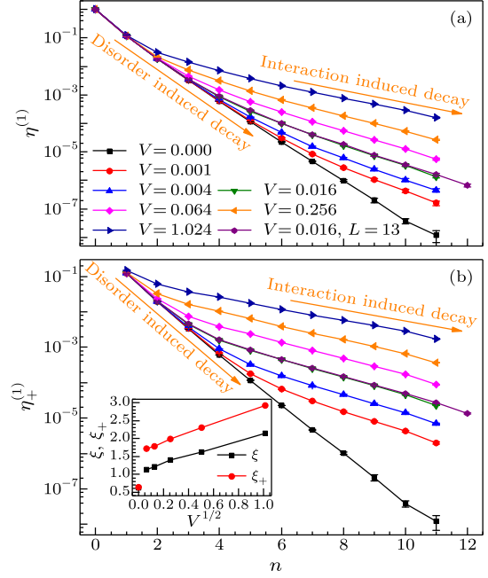
Fig. 1. Disorder averaged reduction errors of (a) the LIOM operator \hat{J}^{(1)} and (b) the corresponding raising operator \hat{J}_+^{(1)} localized near one chain end. We define \eta^{(1)}(n) \equiv \eta_n(\hat{J}^{(1)}) and \eta_+^{(1)}(n) \equiv \eta_n(\hat{J}_+^{(1)}) , in which the target region includes the n sites starting from that chain end. We set the disorder strength w = 32 . The number of lattice sites is L = 12 , except the ones explicitly labeled ( L = 13 ). The exponential decay of the reduction errors have only one phase for V = 0 , which is disorder induced, while the corresponding ones have two phases for V > 0 , featuring the disorder induced decay for small n and the interaction induced decay for large n , respectively. The inset in (b) shows the characteristic lengths extracted from the exponential decays. [36] It is evident that a discontinuity appears at V = 0^+ for both \xi and \xi_+ .
